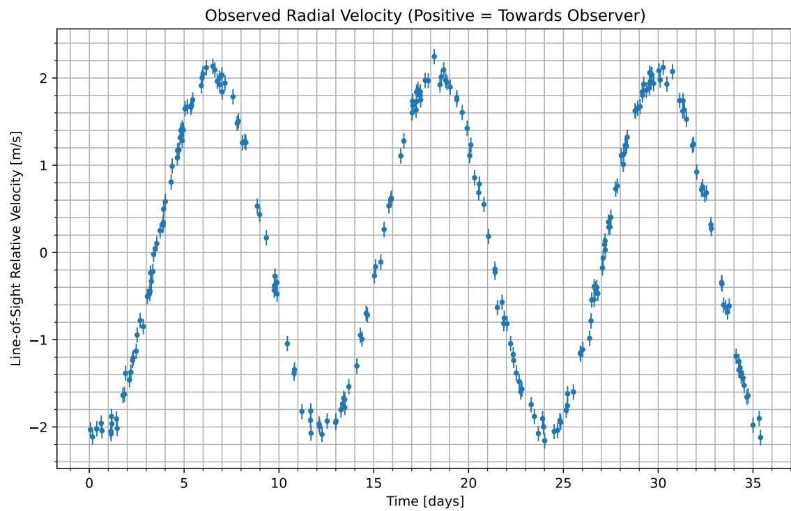
Figure 1: We have isolated the radial velocity of the host star due to the candidate planet. Data begins at UTC 2084-01-15/14:04. Positive values indicate the velocity at which the star is moving towards us; negative indicate the velocity at which it is moving away.
