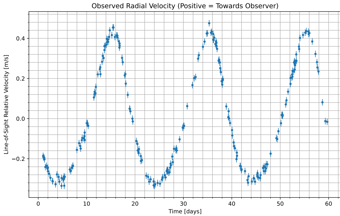
Figure 1: We have isolated the radial velocity of the host star due to the candidate planet. Data begins at UTC 2078-08-05/11:47. Positive values indicate the velocity at which the star is moving towards us; negative indicate the velocity at which it is moving away.
