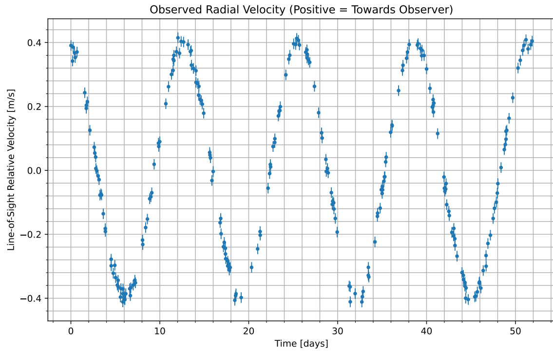
Figure 1: We have isolated the radial velocity of the host star due to the candidate planet. Data begins at UTC 2077-05-23/18:30. Positive values indicate the velocity at which the star is moving towards us; negative indicate the velocity at which it is moving away.
