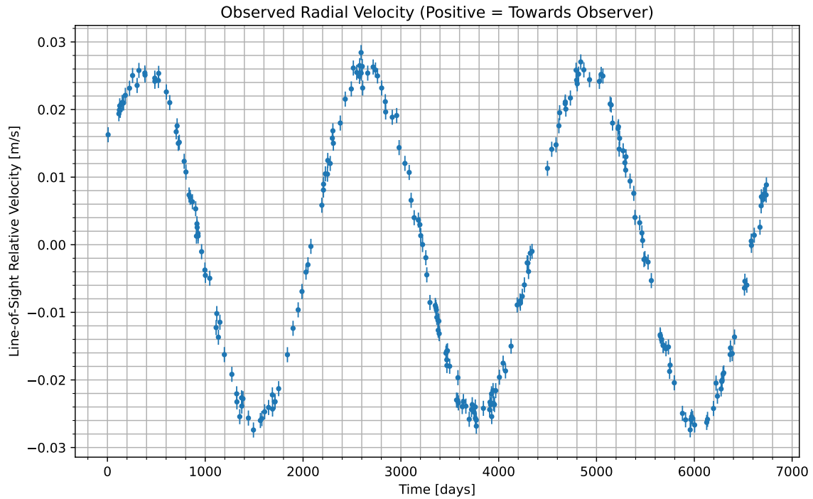
Figure 1: We have isolated the radial velocity of the host star due to the candidate planet. Data begins at UTC 2060-12-10/07:24. Positive values indicate the velocity at which the star is moving towards us; negative indicate the velocity at which it is moving away.
