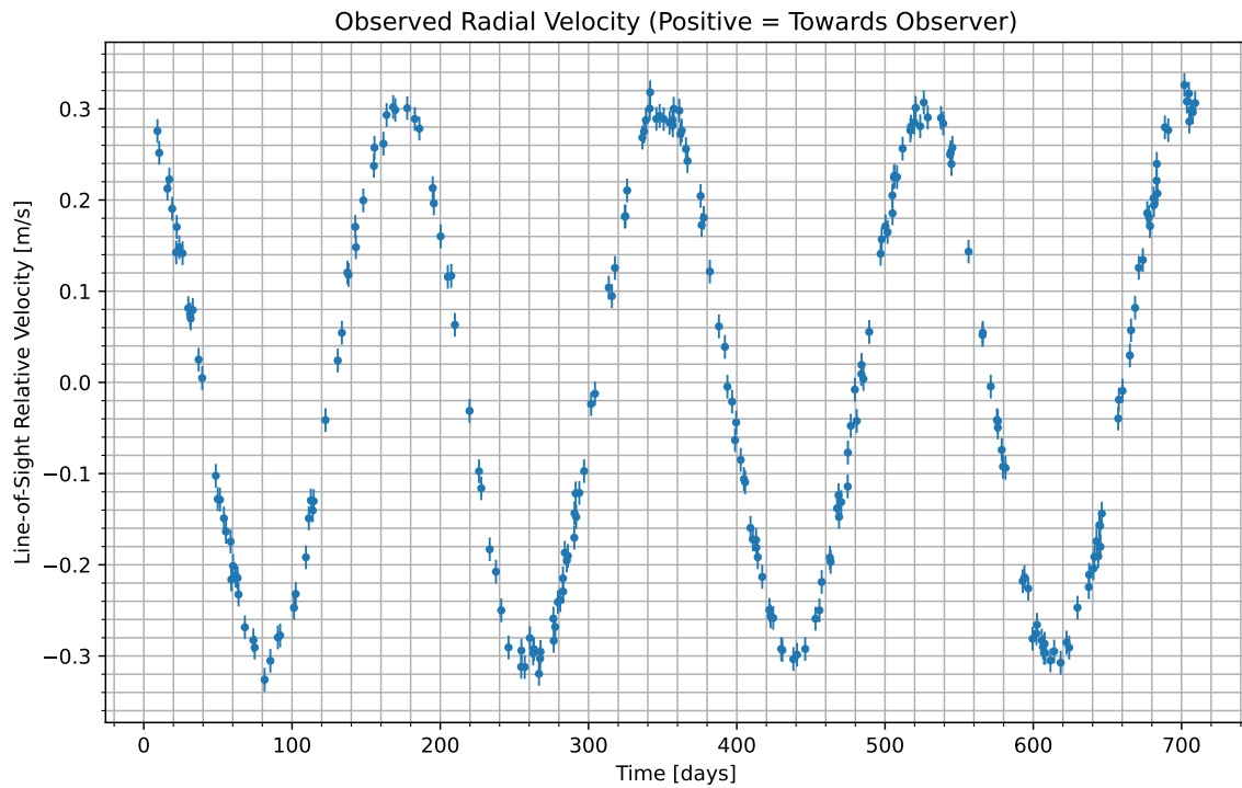
Figure 1: We have isolated the radial velocity of the host star due to the candidate planet. Data begins at UTC 2071-08-24/16:26. Positive values indicate the velocity at which the star is moving towards us; negative indicate the velocity at which it is moving away.
