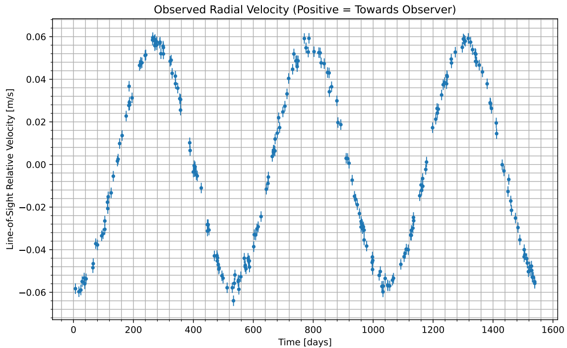
Figure 1: We have isolated the radial velocity of the host star due to the candidate planet. Data begins at UTC 2083-11-11/21:09. Positive values indicate the velocity at which the star is moving towards us; negative indicate the velocity at which it is moving away.
