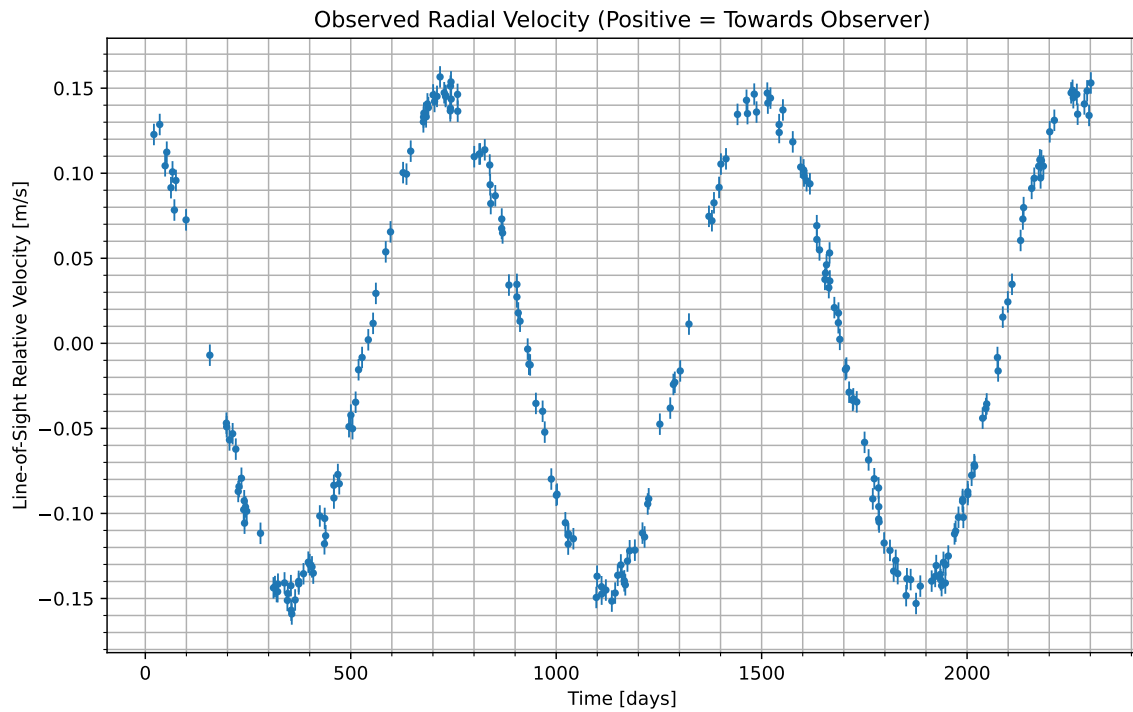
Figure 1: We have isolated the radial velocity of the host star due to the candidate planet. Data begins at UTC 2092-11-26/02:37. Positive values indicate the velocity at which the star is moving towards us; negative indicate the velocity at which it is moving away.
