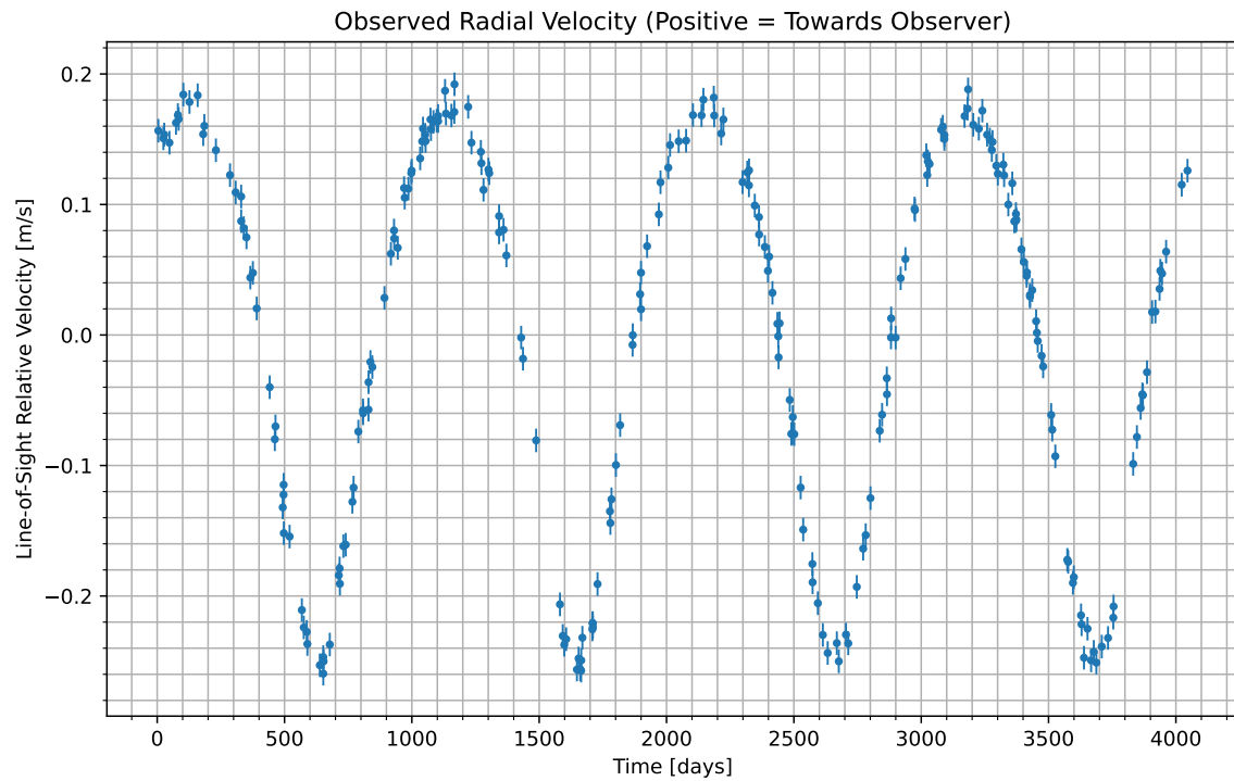
Figure 1: We have isolated the radial velocity of the host star due to the candidate planet. Data begins at UTC 2081-03-06/23:01. Positive values indicate the velocity at which the star is moving towards us; negative indicate the velocity at which it is moving away.
