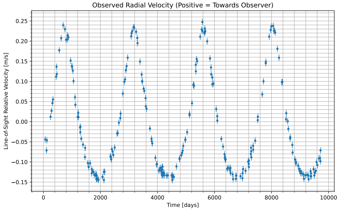
Figure 1: We have isolated the radial velocity of the host star due to the candidate planet. Data begins at UTC 2059-11-09/09:39. Positive values indicate the velocity at which the star is moving towards us; negative indicate the velocity at which it is moving away.
