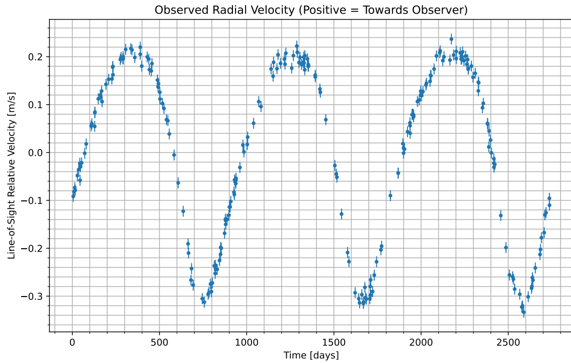
Figure 1: We have isolated the radial velocity of the host star due to the candidate planet. Data begins at UTC 2069-01-03/13:21. Positive values indicate the velocity at which the star is moving towards us; negative indicate the velocity at which it is moving away.
