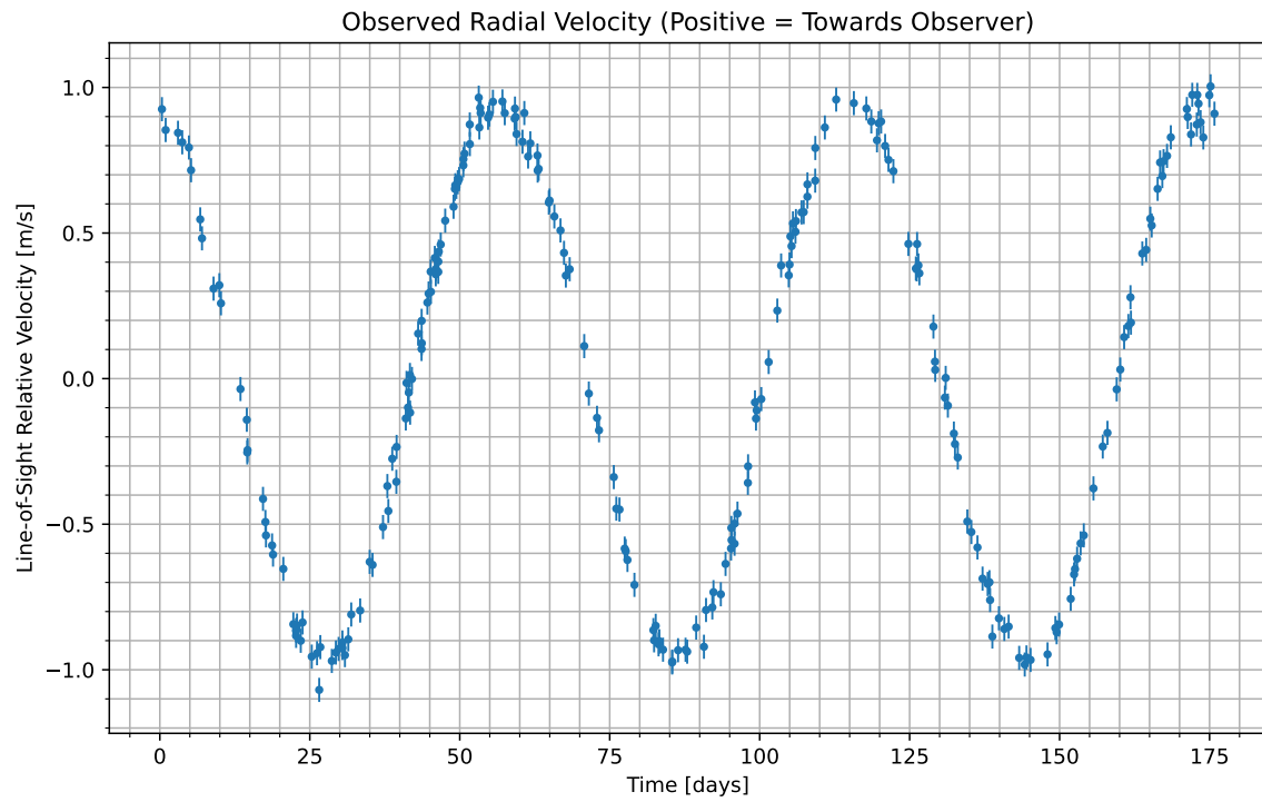
Figure 1: We have isolated the radial velocity of the host star due to the candidate planet. Data begins at UTC 2083-01-29/15:18. Positive values indicate the velocity at which the star is moving towards us; negative indicate the velocity at which it is moving away.
