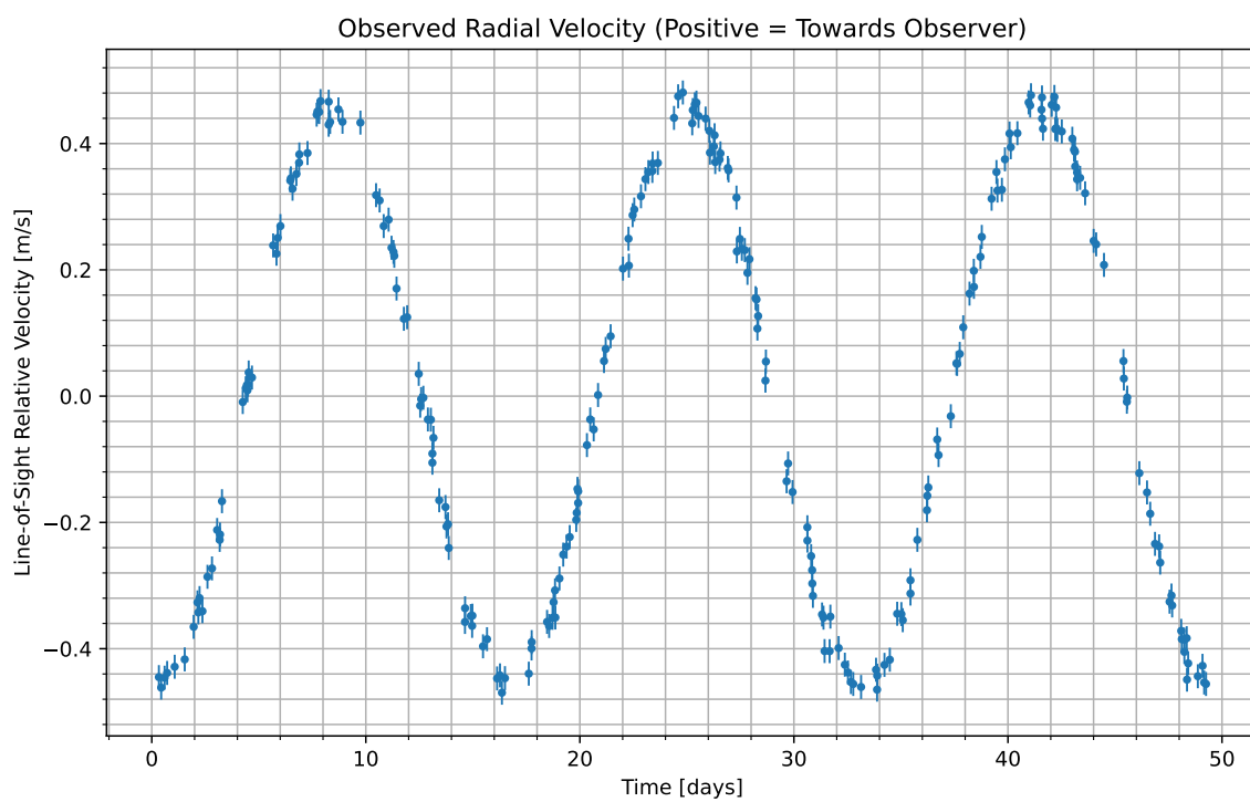
Figure 1: We have isolated the radial velocity of the host star due to the candidate planet. Data begins at UTC 2083-08-05/11:50. Positive values indicate the velocity at which the star is moving towards us; negative indicate the velocity at which it is moving away.
