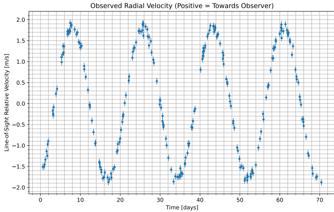
Figure 1: We have isolated the radial velocity of the host star due to the candidate planet. Data begins at UTC 2078-08-22/11:43. Positive values indicate the velocity at which the star is moving towards us; negative indicate the velocity at which it is moving away.
