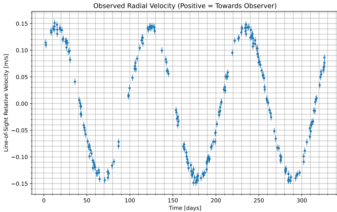
Figure 1: We have isolated the radial velocity of the host star due to the candidate planet. Data begins at UTC 2084-01-24/08:58. Positive values indicate the velocity at which the star is moving towards us; negative indicate the velocity at which it is moving away.
