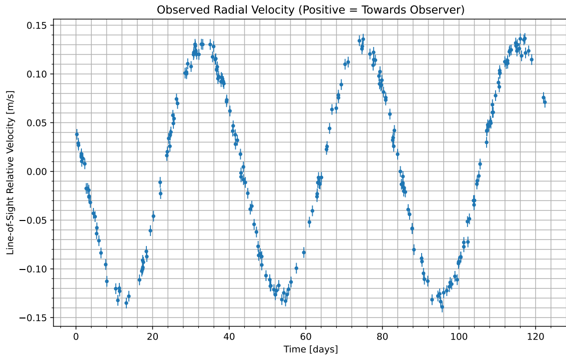
Figure 1: We have isolated the radial velocity of the host star due to the candidate planet. Data begins at UTC 2079-03-17/16:30. Positive values indicate the velocity at which the star is moving towards us; negative indicate the velocity at which it is moving away.
