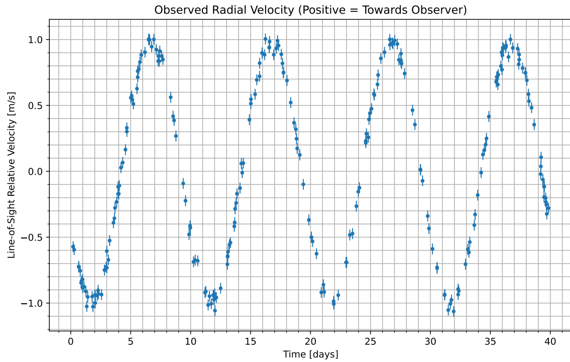
Figure 1: We have isolated the radial velocity of the host star due to the candidate planet. Data begins at UTC 2096-04-08/21:18. Positive values indicate the velocity at which the star is moving towards us; negative indicate the velocity at which it is moving away.
