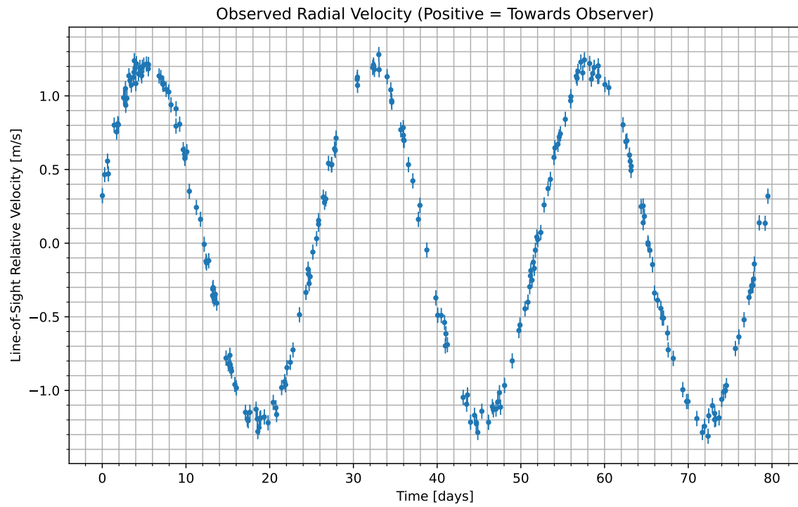
Figure 1: We have isolated the radial velocity of the host star due to the candidate planet. Data begins at UTC 2095-03-20/16:48. Positive values indicate the velocity at which the star is moving towards us; negative indicate the velocity at which it is moving away.
