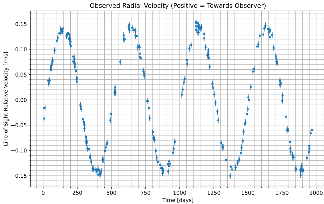
Figure 1: We have isolated the radial velocity of the host star due to the candidate planet. Data begins at UTC 2081-09-29/23:31. Positive values indicate the velocity at which the star is moving towards us; negative indicate the velocity at which it is moving away.
