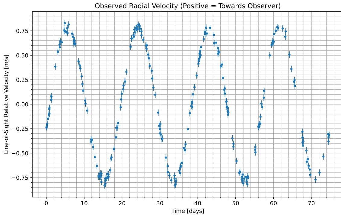
Figure 1: We have isolated the radial velocity of the host star due to the candidate planet. Data begins at UTC 2096-10-21/23:36. Positive values indicate the velocity at which the star is moving towards us; negative indicate the velocity at which it is moving away.
