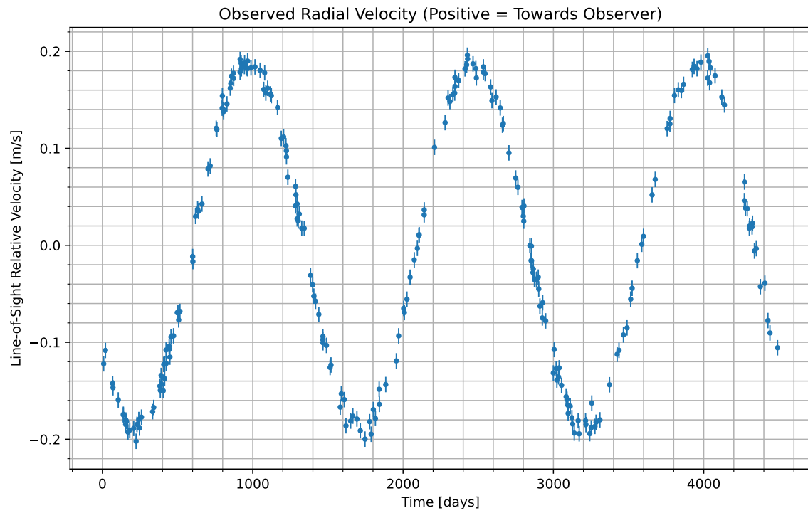
Figure 1: We have isolated the radial velocity of the host star due to the candidate planet. Data begins at UTC 2061-10-19/13:47. Positive values indicate the velocity at which the star is moving towards us; negative indicate the velocity at which it is moving away.
