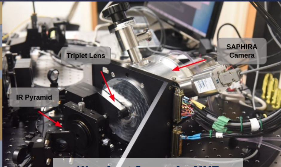
Wavefront Sensor for MMT
