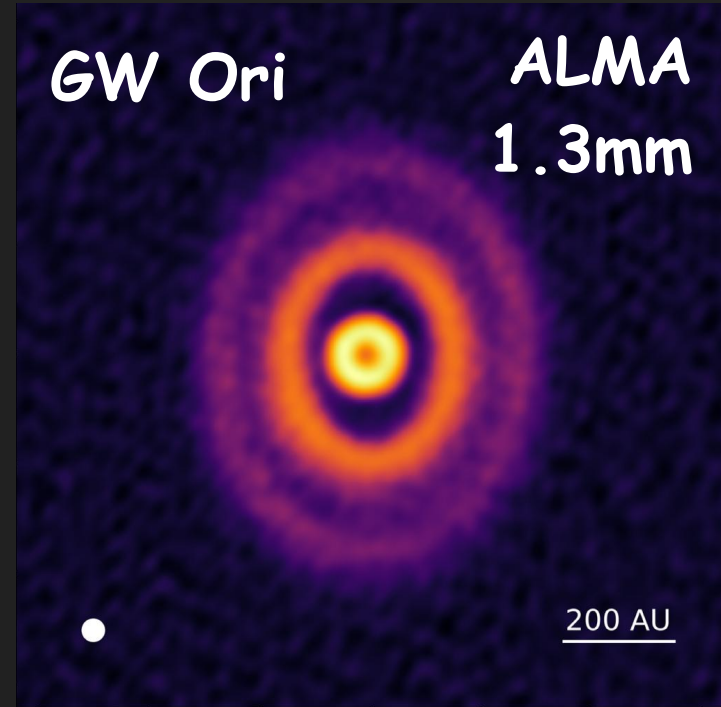
Misaligned Planet-Forming Rings around Triple Young Stars (Bi et al., 2020)
