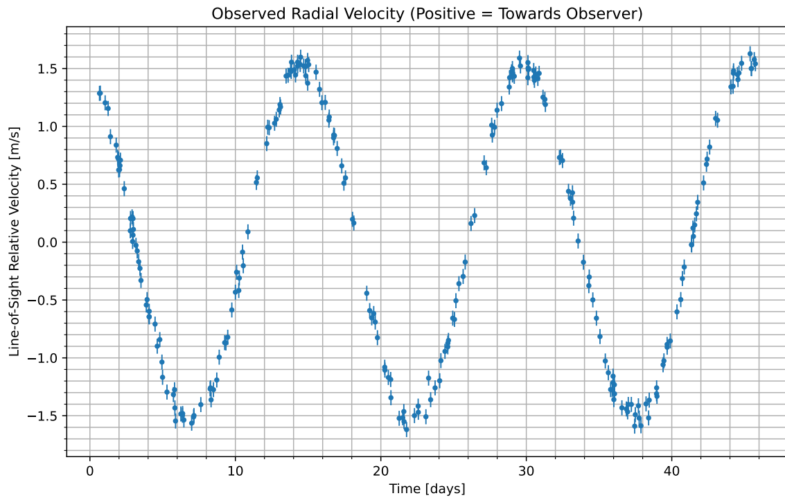
Figure 1: We have isolated the radial velocity of the host star due to the candidate planet. Data begins at UTC 2075-12-09/23:36. Positive values indicate the velocity at which the star is moving towards us; negative indicate the velocity at which it is moving away.
