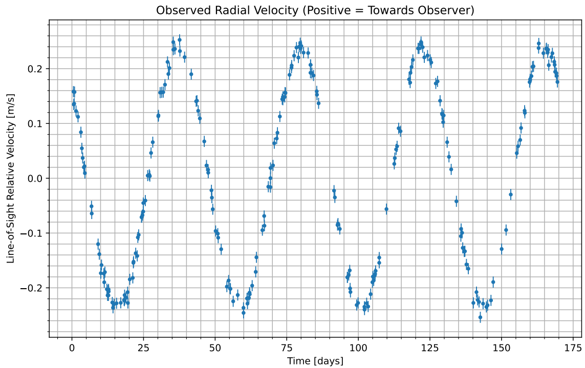
Figure 1: We have isolated the radial velocity of the host star due to the candidate planet. Data begins at UTC 2089-10-27/14:55. Positive values indicate the velocity at which the star is moving towards us; negative indicate the velocity at which it is moving away.
