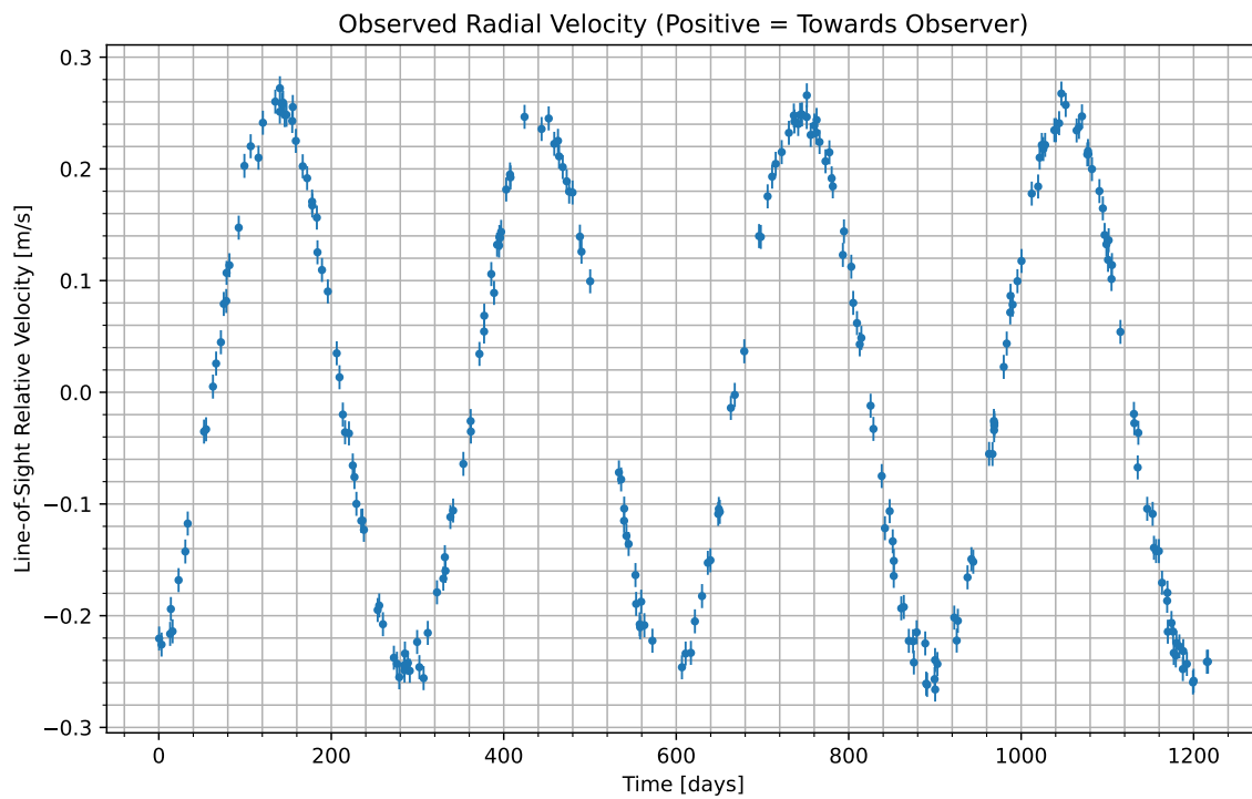
Figure 1: We have isolated the radial velocity of the host star due to the candidate planet. Data begins at UTC 2075-10-10/23:37. Positive values indicate the velocity at which the star is moving towards us; negative indicate the velocity at which it is moving away.
