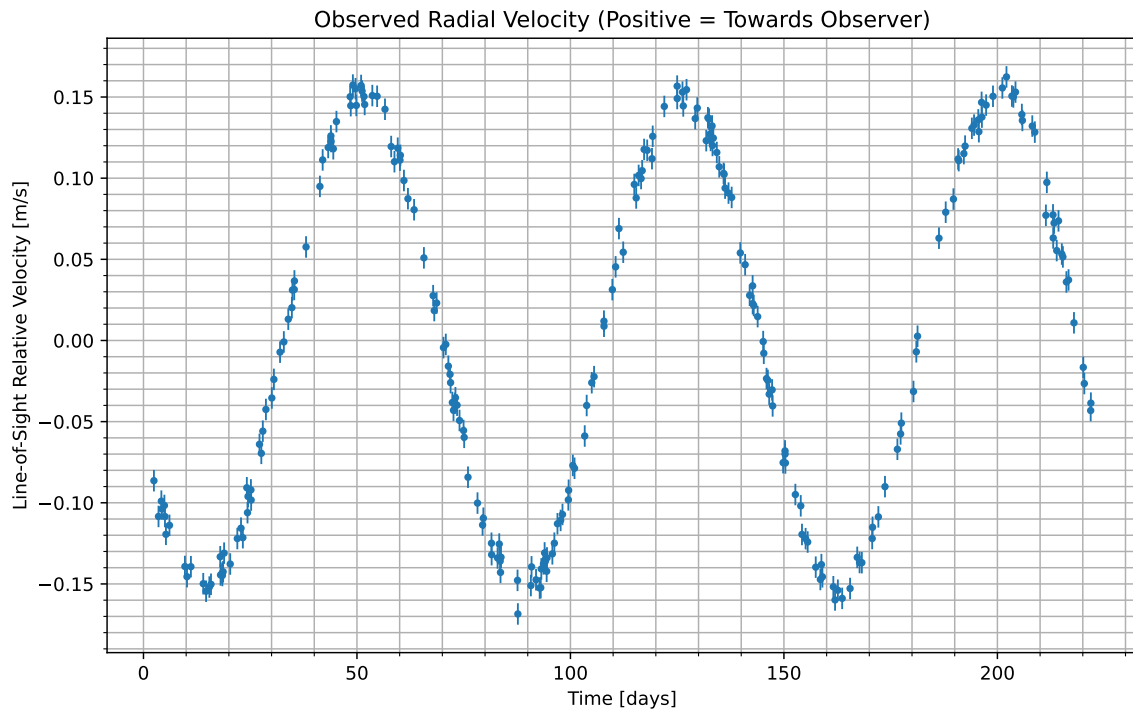
Figure 1: We have isolated the radial velocity of the host star due to the candidate planet. Data begins at UTC 2085-08-03/14:37. Positive values indicate the velocity at which the star is moving towards us; negative indicate the velocity at which it is moving away.
