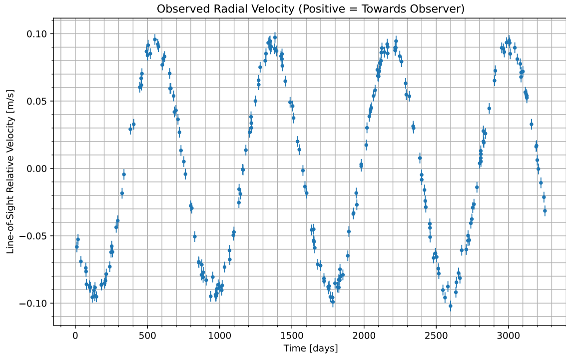
Figure 1: We have isolated the radial velocity of the host star due to the candidate planet. Data begins at UTC 2076-02-06/21:46. Positive values indicate the velocity at which the star is moving towards us; negative indicate the velocity at which it is moving away.
