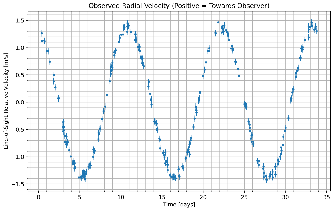
Figure 1: We have isolated the radial velocity of the host star due to the candidate planet. Data begins at UTC 2077-02-03/23:25. Positive values indicate the velocity at which the star is moving towards us; negative indicate the velocity at which it is moving away.
