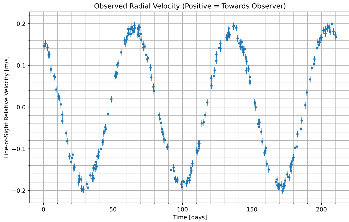
Figure 1: We have isolated the radial velocity of the host star due to the candidate planet. Data begins at UTC 2098-03-18/06:41. Positive values indicate the velocity at which the star is moving towards us; negative indicate the velocity at which it is moving away.
