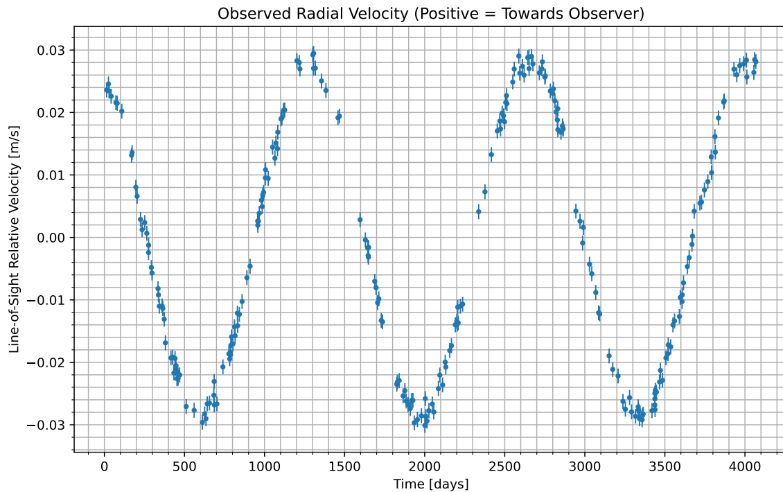
Figure 1: We have isolated the radial velocity of the host star due to the candidate planet. Data begins at UTC 2080-12-29/20:21. Positive values indicate the velocity at which the star is moving towards us; negative indicate the velocity at which it is moving away.
