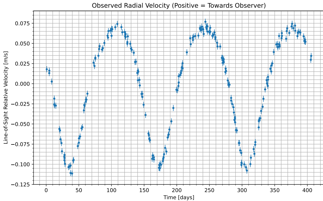
Figure 1: We have isolated the radial velocity of the host star due to the candidate planet. Data begins at UTC 2094-07-31/22:41. Positive values indicate the velocity at which the star is moving towards us; negative indicate the velocity at which it is moving away.
