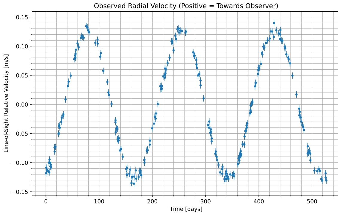
Figure 1: We have isolated the radial velocity of the host star due to the candidate planet. Data begins at UTC 2098-04-20/08:10. Positive values indicate the velocity at which the star is moving towards us; negative indicate the velocity at which it is moving away.
