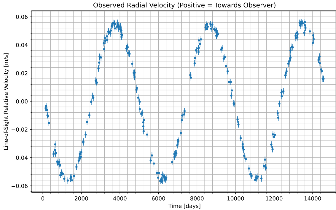
Figure 1: We have isolated the radial velocity of the host star due to the candidate planet. Data begins at UTC 2035-09-08/07:42. Positive values indicate the velocity at which the star is moving towards us; negative indicate the velocity at which it is moving away.
