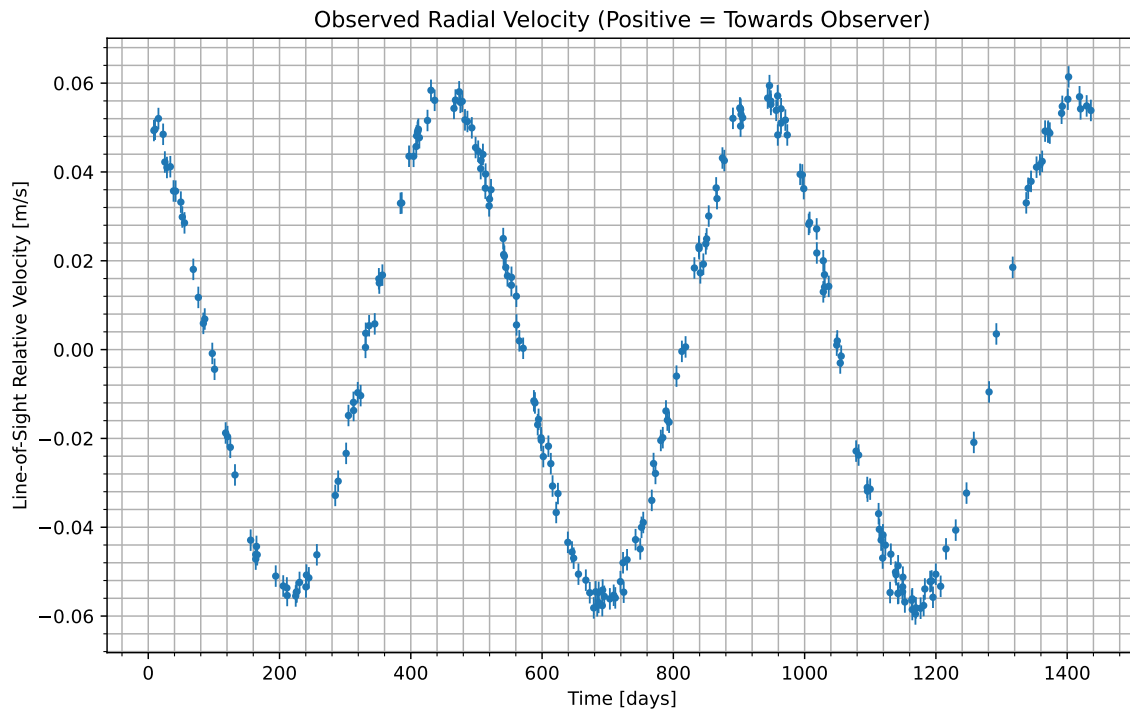
Figure 1: We have isolated the radial velocity of the host star due to the candidate planet. Data begins at UTC 2072-09-02/13:42. Positive values indicate the velocity at which the star is moving towards us; negative indicate the velocity at which it is moving away.
