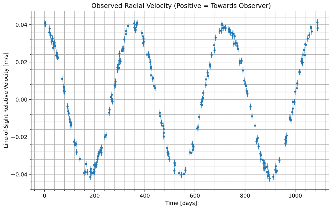
Figure 1: We have isolated the radial velocity of the host star due to the candidate planet. Data begins at UTC 2081-11-23/13:26. Positive values indicate the velocity at which the star is moving towards us; negative indicate the velocity at which it is moving away.
