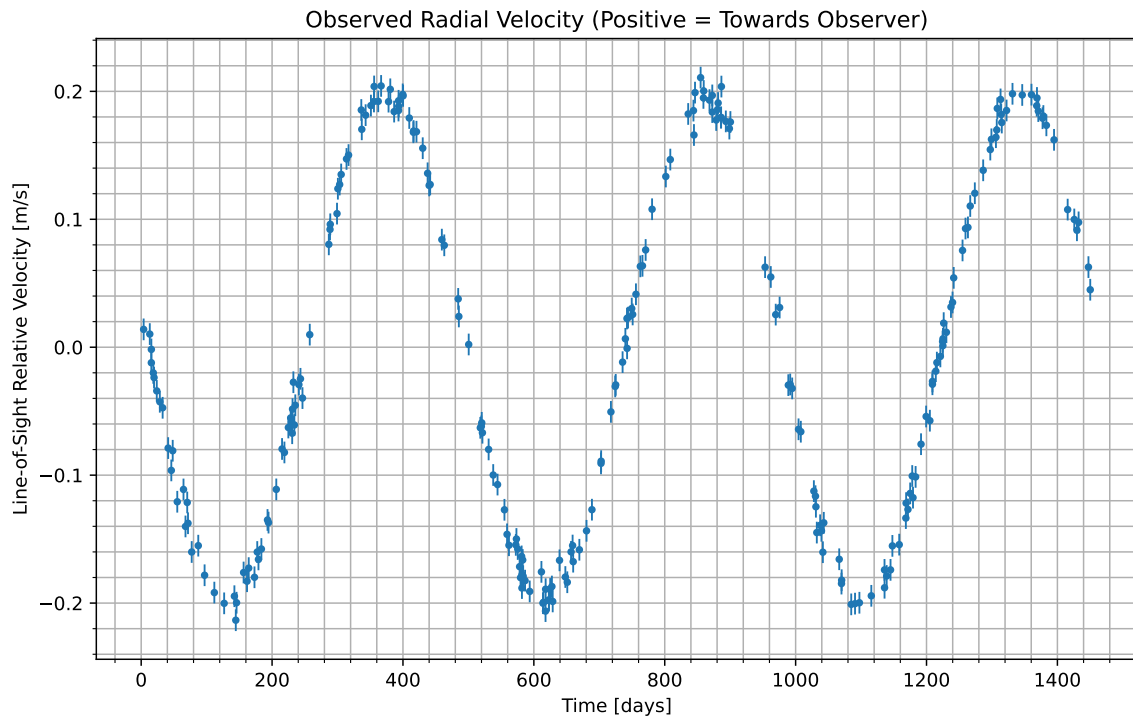
Figure 1: We have isolated the radial velocity of the host star due to the candidate planet. Data begins at UTC 2073-10-22/14:31. Positive values indicate the velocity at which the star is moving towards us; negative indicate the velocity at which it is moving away.
