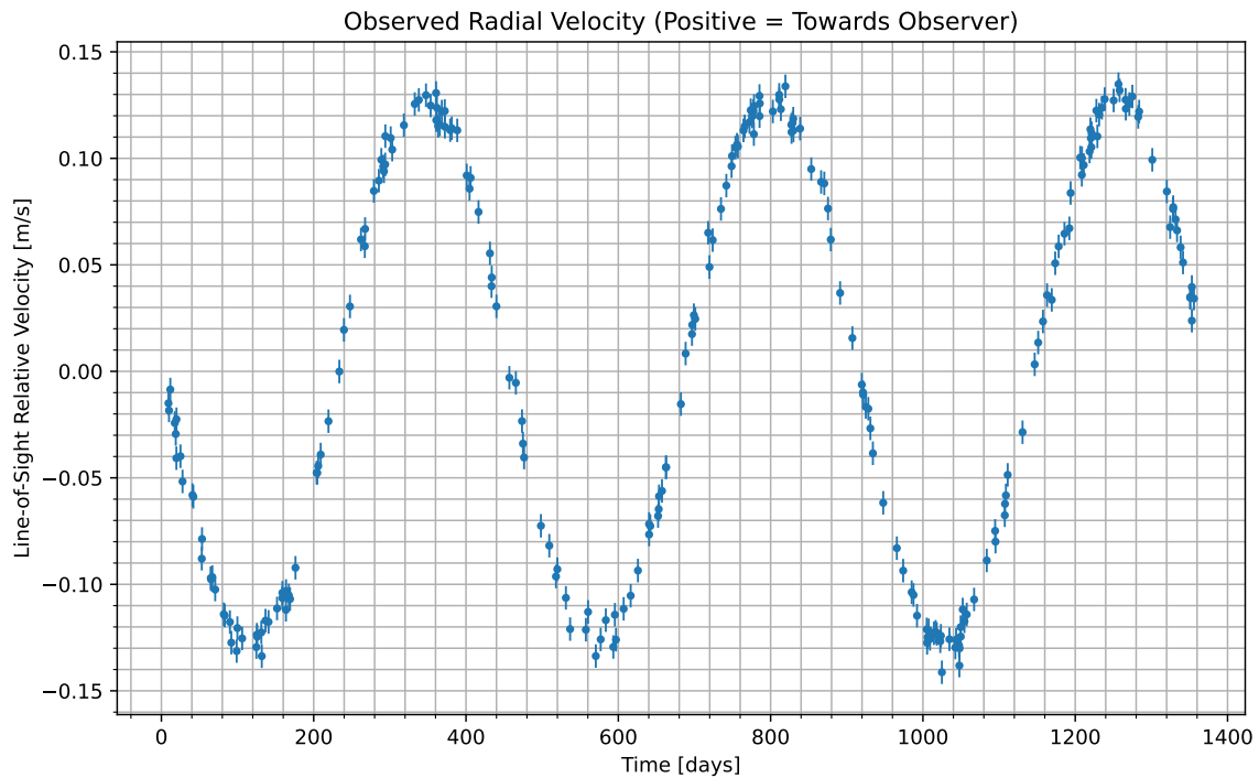
Figure 1: We have isolated the radial velocity of the host star due to the candidate planet. Data begins at UTC 2092-08-30/19:26. Positive values indicate the velocity at which the star is moving towards us; negative indicate the velocity at which it is moving away.
