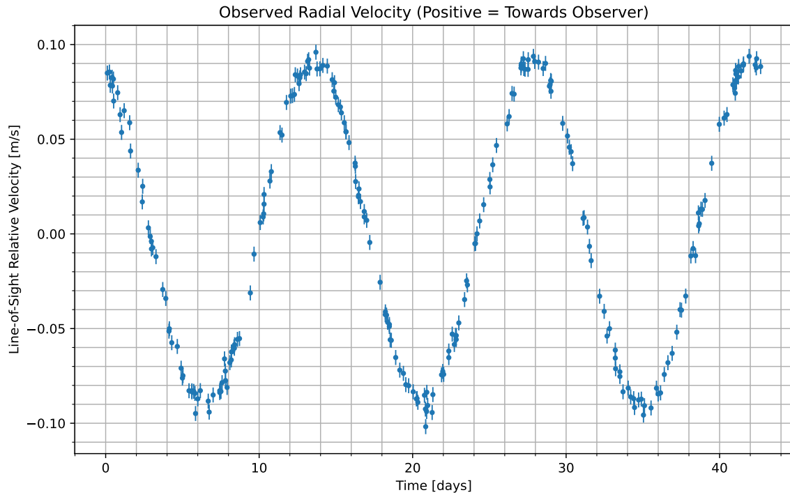
Figure 1: We have isolated the radial velocity of the host star due to the candidate planet. Data begins at UTC 2074-09-03/23:00. Positive values indicate the velocity at which the star is moving towards us; negative indicate the velocity at which it is moving away.
