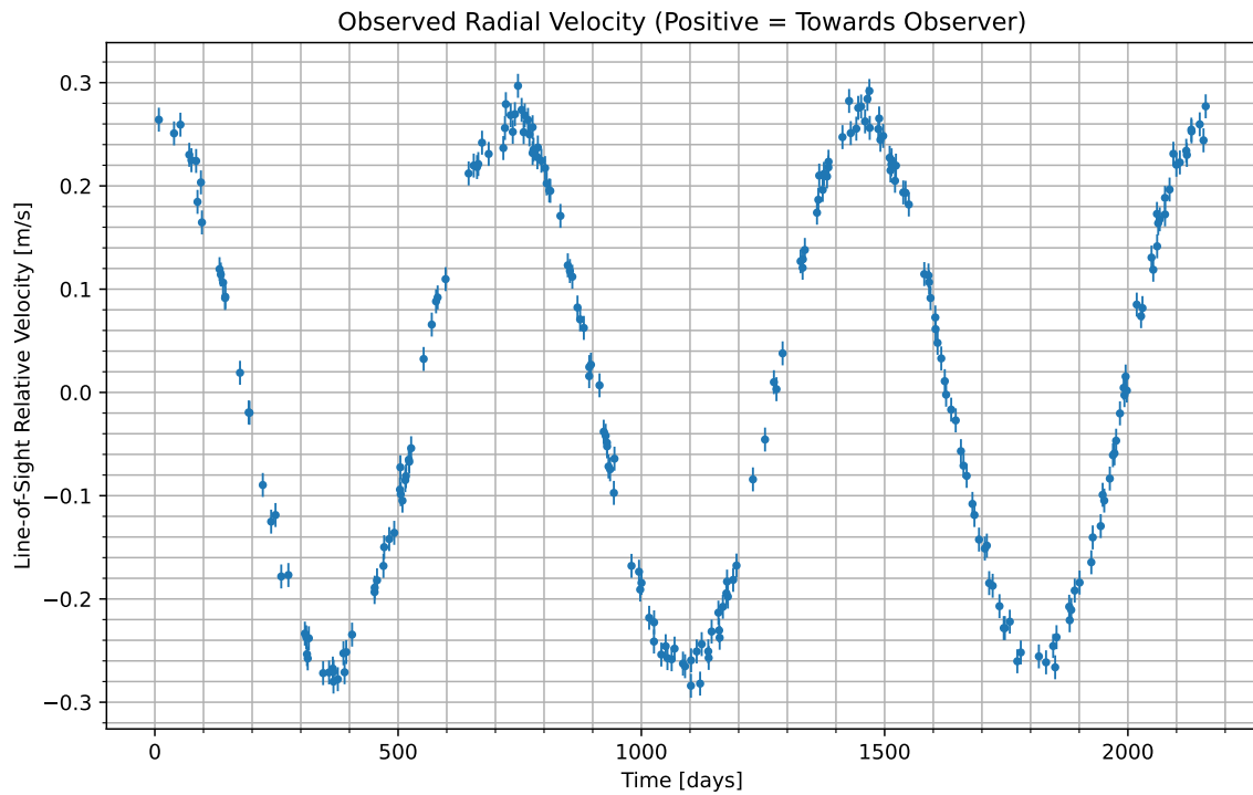
Figure 1: We have isolated the radial velocity of the host star due to the candidate planet. Data begins at UTC 2093-01-17/10:25. Positive values indicate the velocity at which the star is moving towards us; negative indicate the velocity at which it is moving away.
