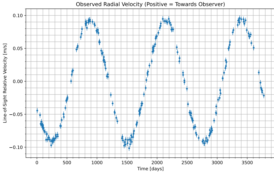
Figure 1: We have isolated the radial velocity of the host star due to the candidate planet. Data begins at UTC 2061-06-18/10:36. Positive values indicate the velocity at which the star is moving towards us; negative indicate the velocity at which it is moving away.
