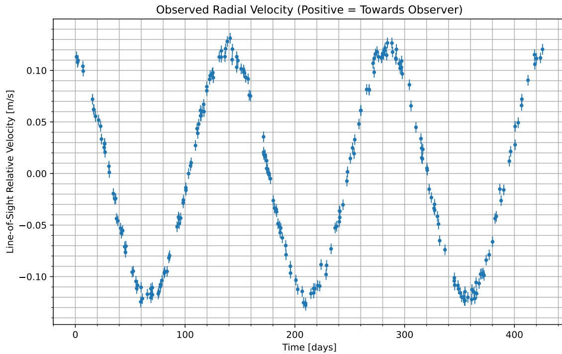
Figure 1: We have isolated the radial velocity of the host star due to the candidate planet. Data begins at UTC 2081-04-27/04:29. Positive values indicate the velocity at which the star is moving towards us; negative indicate the velocity at which it is moving away.
