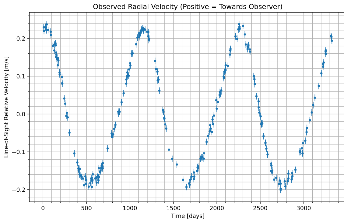
Figure 1: We have isolated the radial velocity of the host star due to the candidate planet. Data begins at UTC 2062-07-17/12:39. Positive values indicate the velocity at which the star is moving towards us; negative indicate the velocity at which it is moving away.
