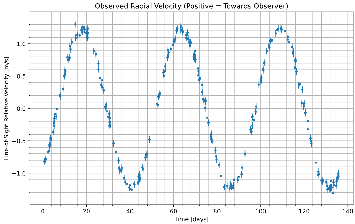
Figure 1: We have isolated the radial velocity of the host star due to the candidate planet. Data begins at UTC 2089-05-17/10:29. Positive values indicate the velocity at which the star is moving towards us; negative indicate the velocity at which it is moving away.
