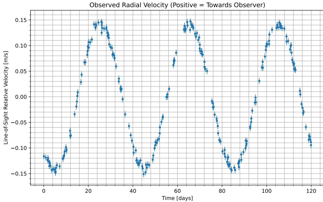
Figure 1: We have isolated the radial velocity of the host star due to the candidate planet. Data begins at UTC 2070-12-31/18:05. Positive values indicate the velocity at which the star is moving towards us; negative indicate the velocity at which it is moving away.
