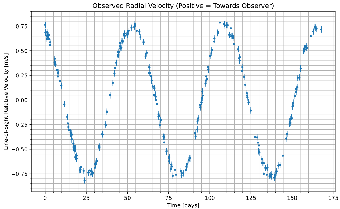
Figure 1: We have isolated the radial velocity of the host star due to the candidate planet. Data begins at UTC 2094-08-22/18:30. Positive values indicate the velocity at which the star is moving towards us; negative indicate the velocity at which it is moving away.
