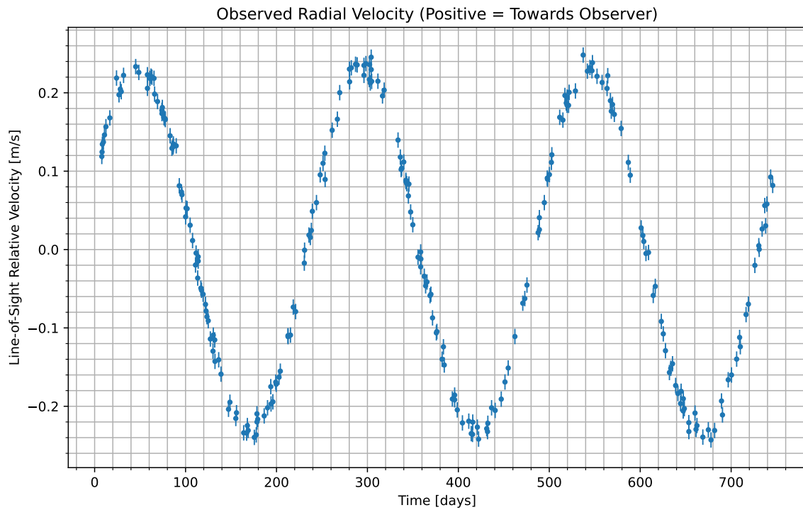
Figure 1: We have isolated the radial velocity of the host star due to the candidate planet. Data begins at UTC 2088-06-15/03:04. Positive values indicate the velocity at which the star is moving towards us; negative indicate the velocity at which it is moving away.
