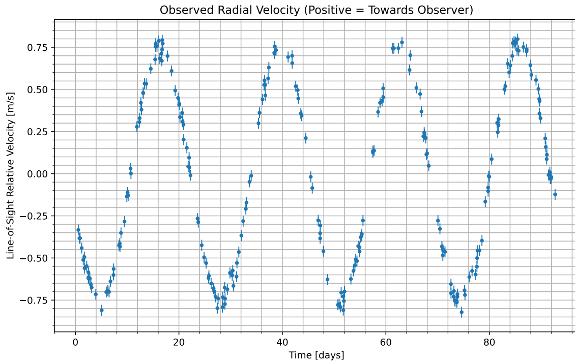
Figure 1: We have isolated the radial velocity of the host star due to the candidate planet. Data begins at UTC 2097-07-06/11:08. Positive values indicate the velocity at which the star is moving towards us; negative indicate the velocity at which it is moving away.
