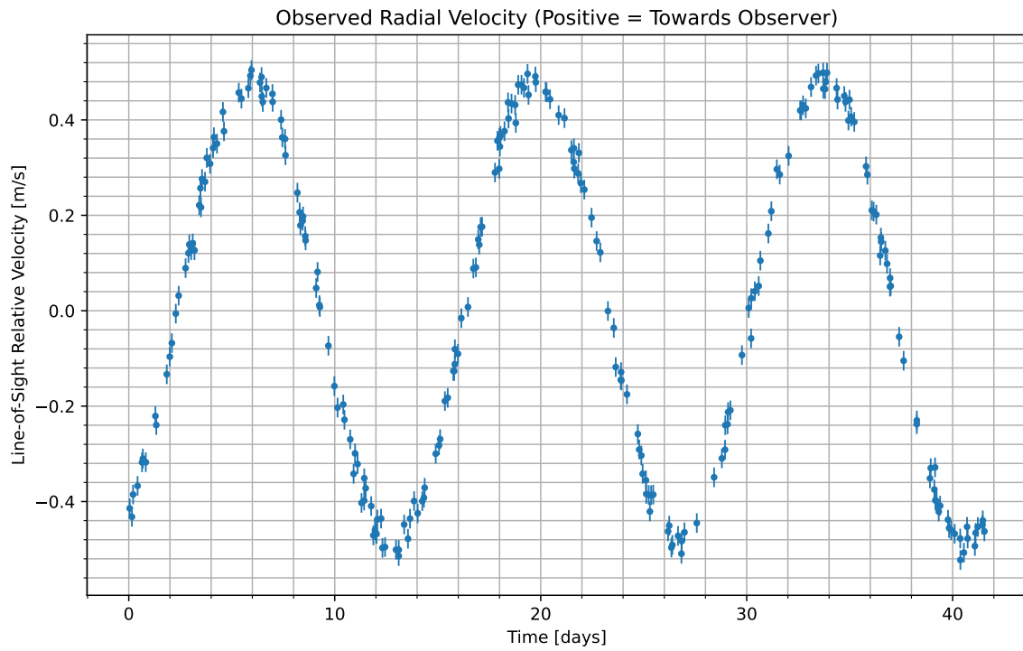
Figure 1: We have isolated the radial velocity of the host star due to the candidate planet. Data begins at UTC 2092-08-02/02:02. Positive values indicate the velocity at which the star is moving towards us; negative indicate the velocity at which it is moving away.
