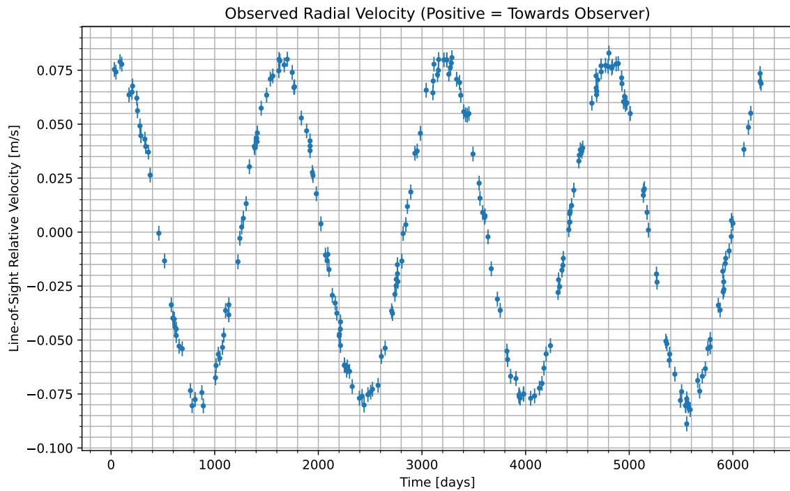
Figure 1: We have isolated the radial velocity of the host star due to the candidate planet. Data begins at UTC 2065-06-24/21:25. Positive values indicate the velocity at which the star is moving towards us; negative indicate the velocity at which it is moving away.
