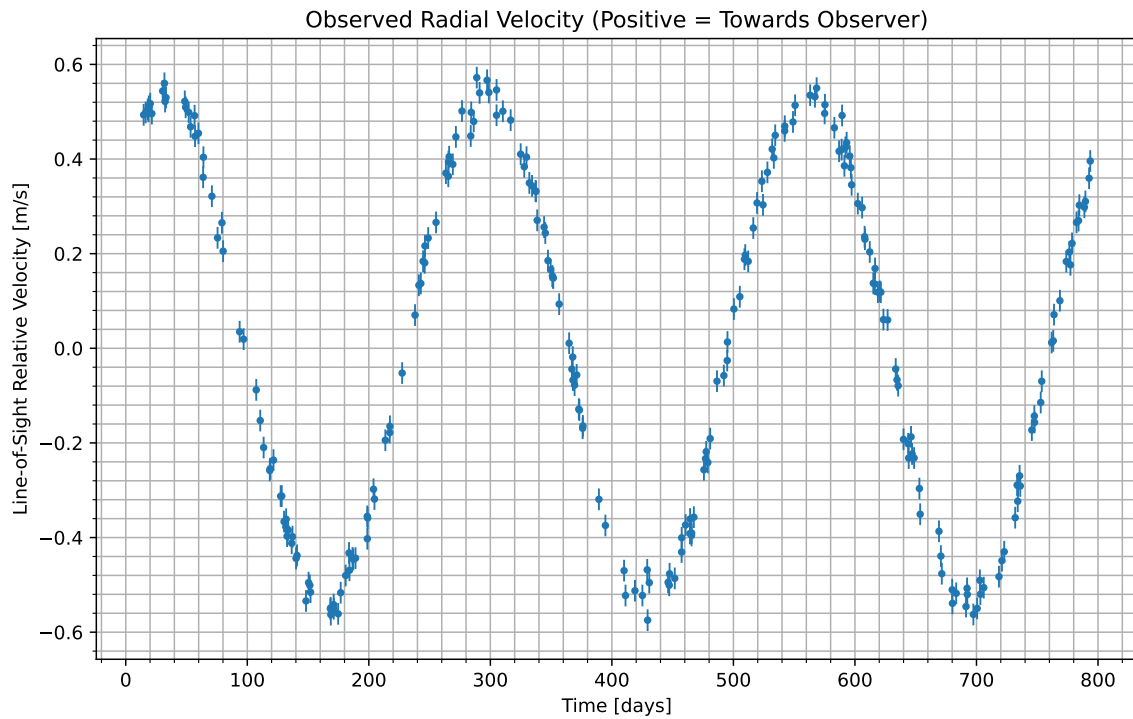
Figure 1: We have isolated the radial velocity of the host star due to the candidate planet. Data begins at UTC 2095-02-05/02:58. Positive values indicate the velocity at which the star is moving towards us; negative indicate the velocity at which it is moving away.
